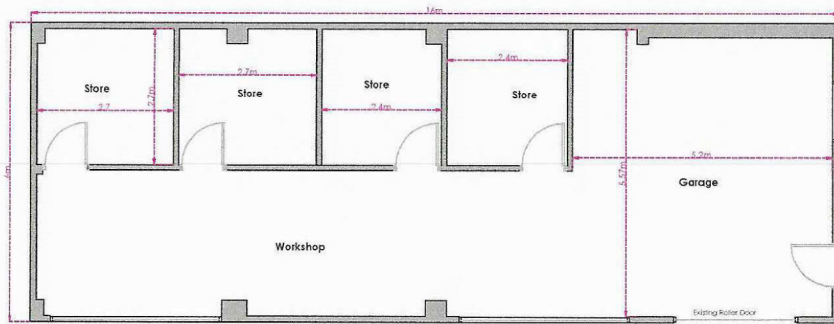
Proposed Workshop / Garage Plans 1:50
